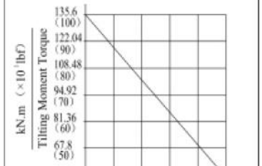
MOMENT LOAD CHART
